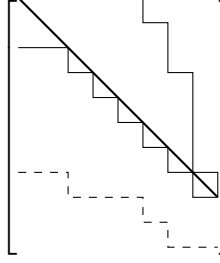
Figure 3.2: The generic picture for paths in the proof of Theorem 2. The lower two paths are examples of the two possible cases.
