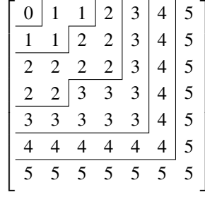
Figure 3.3: The contiguous regions of a Hardinian array are separated by a tuple of nonintersecting lattice walks starting on the left and ending at the top.
