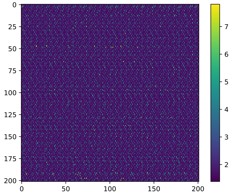
Figure 4.1: Log-heatmap of the first pseudoprime of x^2 - ax - b .
