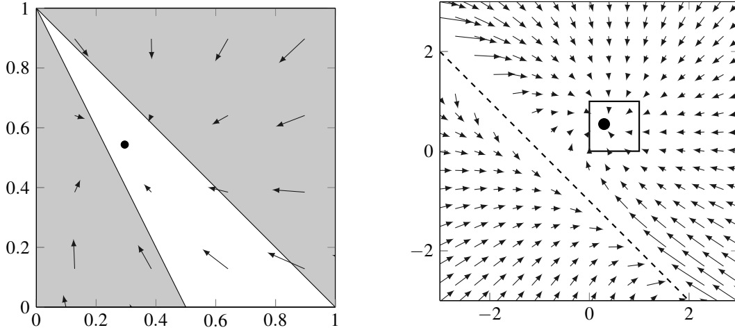
Figure 5.1: The map (x, y, z) \mapsto (y, z, x + y + z) represented in the ts plane by its equivalent (t, s) \mapsto (s/(s + t + 1), 1/(s + t + 1)) . Left: The map restricted to the unit square, with the region \{s + t > 1\} \cup \{s + 2t < 1\} shaded. The unique critical point in the first quadrant of the left-hand side of (5.4) is labeled by a black dot. Right: The map on a larger portion of the plane. The critical point is an attractor for s + t + 1 > 0 .
