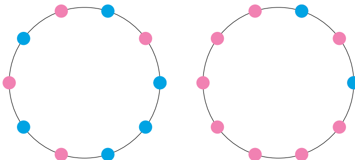
Figure 1.1: Left: A valid array of size 10. Right: An invalid array of size 10.
