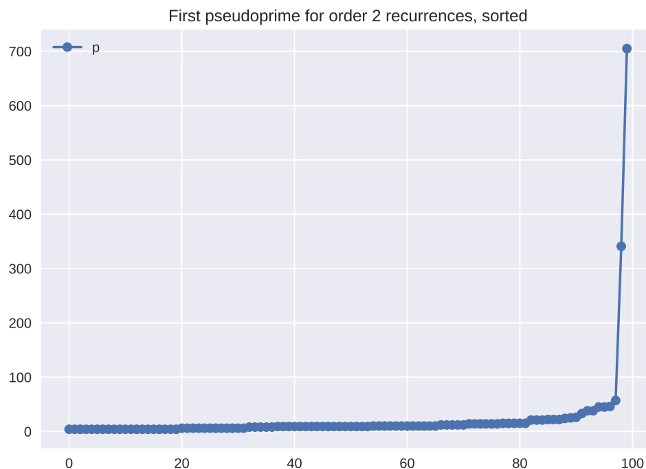
Figure 4.2: Sorted first pseudoprime of x^2 - ax - b
