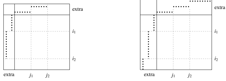
Figure 3.4: Left: the computation of \sum_{i_1 < i_2 < i_3 < i_4} \sum_{j_1 < j_2 < j_3 < j_4} \Delta(n-1)_{i_1, i_2, i_3, i_4}^{j_1, j_2, j_3, j_4} is equivalent to the computation of the sum over i_1, i_2 and j_1, j_2 of the determinants constructed as shown in the figure. Light dots indicated omitted rows and columns; strong dots indicate regions filled with alternating signs. Right: the computation of \sum_{i_1 < i_2 < i_3 < i_4 < i_5} \sum_{j_1 < j_2 < j_3 < j_4 < j_5} \Delta(n-1)_{i_1, i_2, i_3, i_4, i_5}^{j_1, j_2, j_3, j_4, j_5} is equivalent to the computation of the sum over i_1, i_2 and j_1, j_2 of the determinants constructed as shown in the figure.
