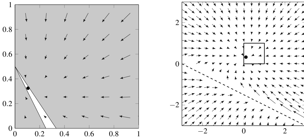
Figure 5.2: The map (x, y, z) \mapsto (y, z, 3z + 2y + x) represented in the ts plane by its equivalent (t, s) \mapsto (s/(2s + t + 3), 1/(2s + t + 3)) . Left: The map restricted to the unit square, with the region \{2s + 3t \geq 1\} \cup \{2s + 4t \leq 1\} shaded. The unique critical point in the first quadrant of the cubic constructed in the proof of Proposition 13 with parameters (a, b) = (2, 3) is labeled by a black dot. Right: The map on a larger portion of the plane.
